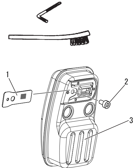
1. Spark arrestor screen
