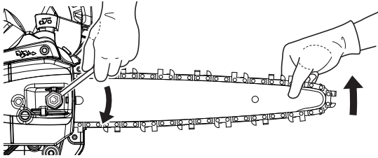
1. Chain tension adjuster 2. Direction to tension the chain
