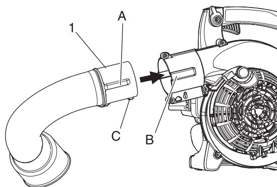
1. Vacuum elbow
